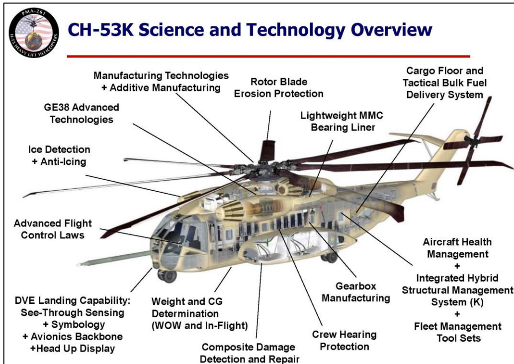
Figure F-4 CH-53K Science and Technology
